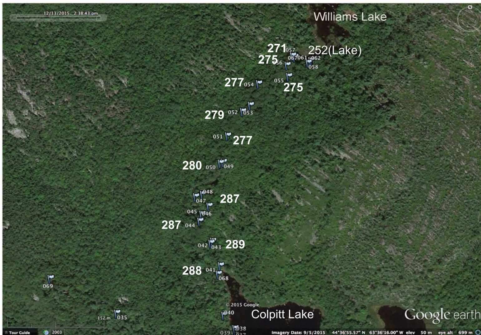
Fig. 5. Specific Conductance values ( \mu\text{S}/\text{cm} ) on the stream running between Colpitt Lake and Williams Lake on Dec 13, 2015.
